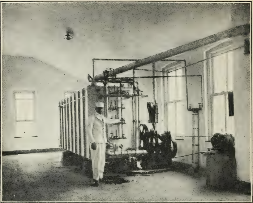
FIG. 11.—In-the-bottle pasteurizer, showing pumps which force the sprays of hot water over the bottles.
